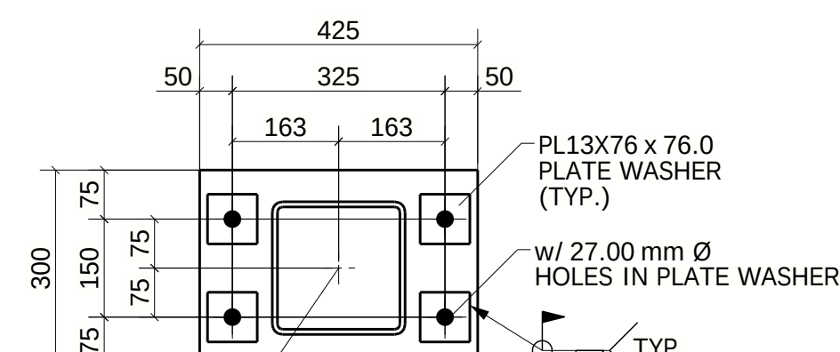
TYPE-03 (12-LOCATION) (REF : PB-5/S-170)
