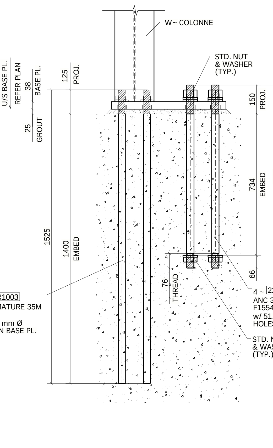
TYPE-13 (01-LOCATION) (REF : PB-1-D-4/S-170)
