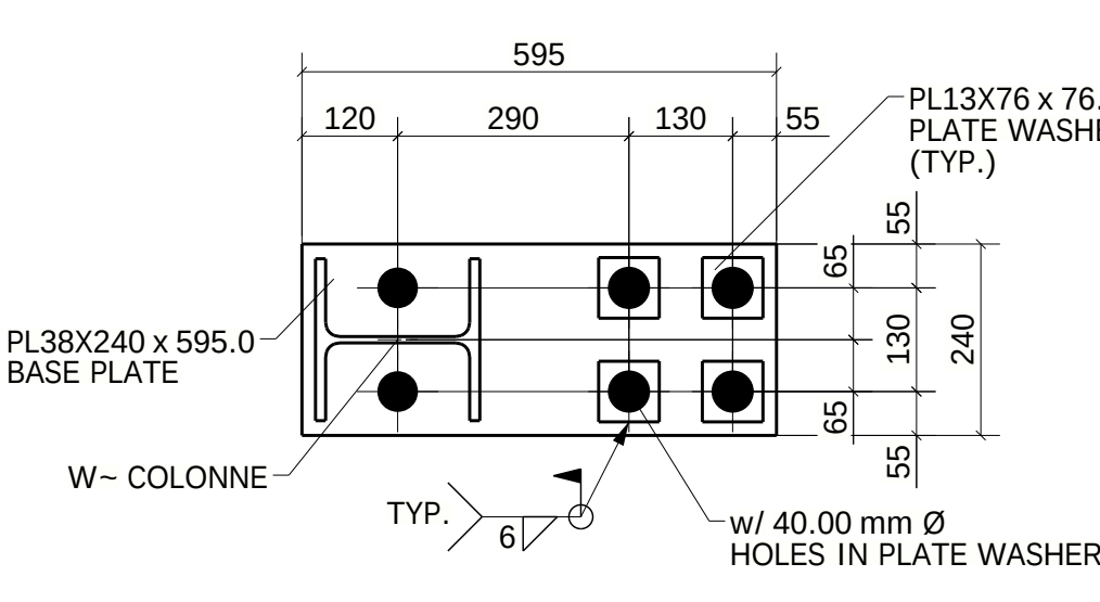
TYPE-13A (05-LOCATIONS) (REF : PB-1-D-4/S-170)
