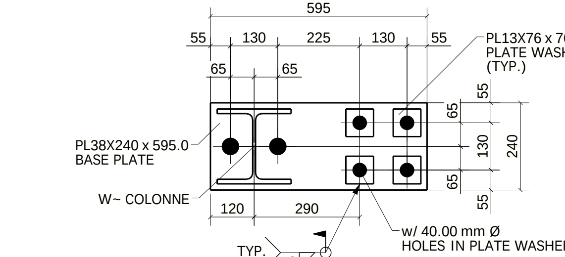
TYPE-18 (03-LOCATIONS) (REF : PB-1-C-4/S-170)
