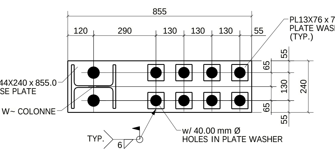
TYPE-17 (04-LOCATIONS) (REF : PB-1-E-8/S-170)
