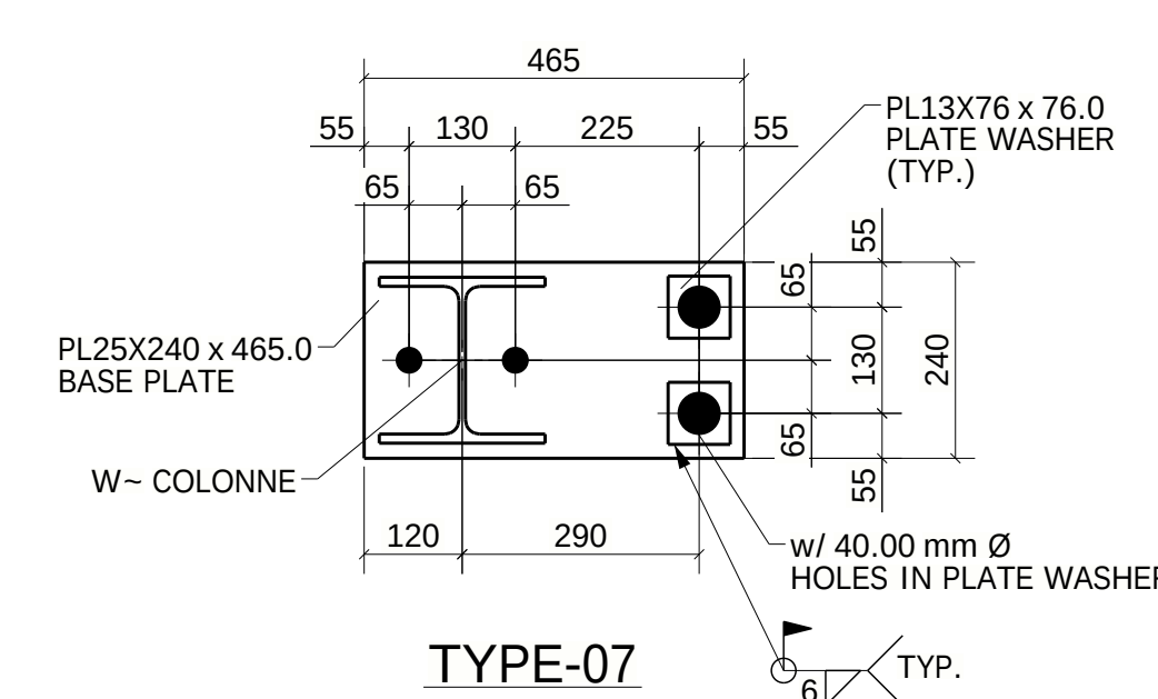
TYPE-07 (04-LOCATION) (REF : PB-1-A-2/S-170)
