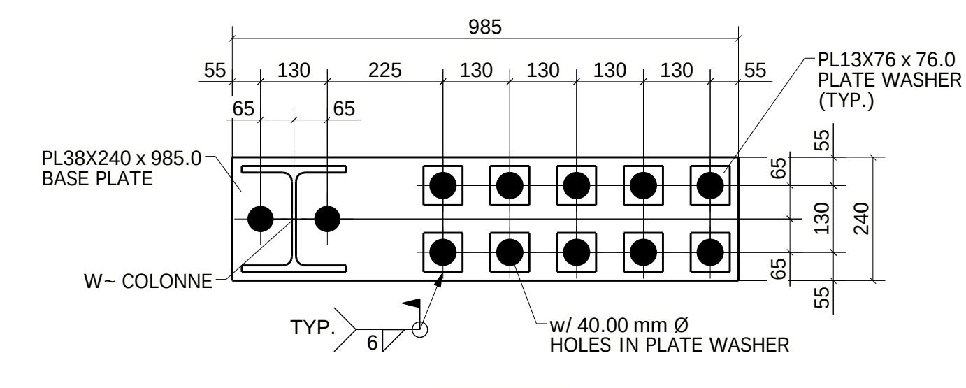
TYPE-15 (01-LOCATION) (REF : PB-1-D-10/S-170)
