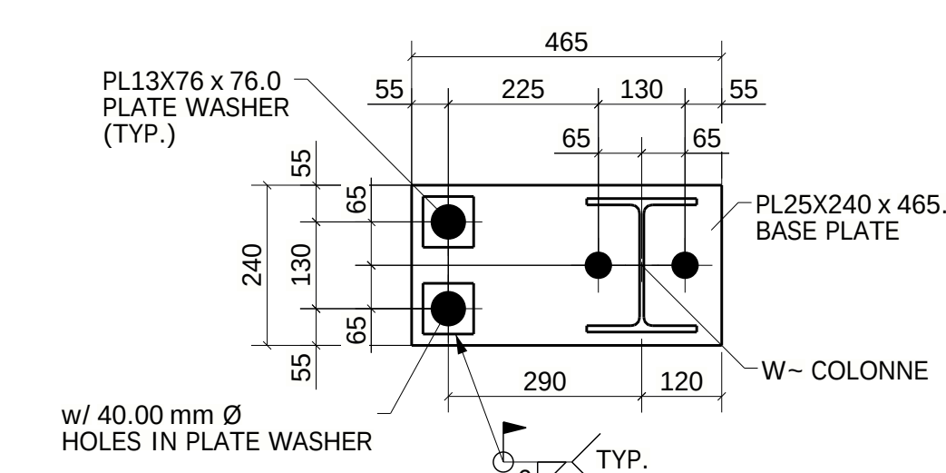
TYPE-09 (02-LOCATION) (REF : PB-1-B-2/S-170)
