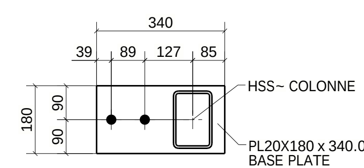
TYPE-04 (06-LOCATION) (REF : PB-6/S-170)
