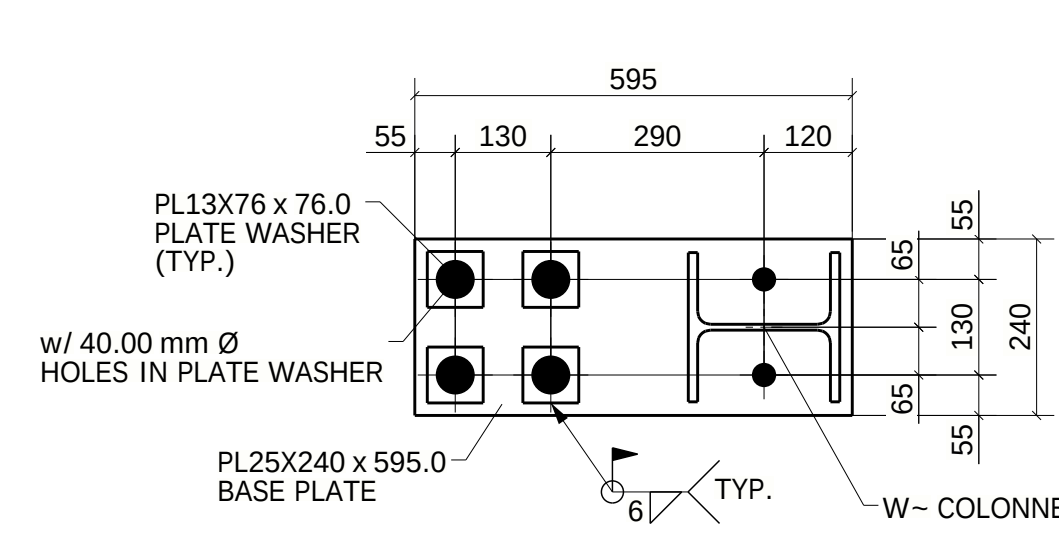
TYPE-08A (08-LOCATION) (REF : PB-1-A-4/S-170)
