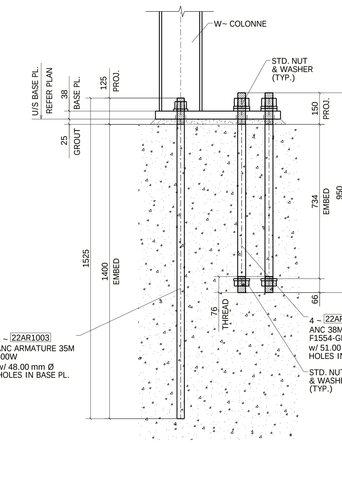
TYPE-13A (05-LOCATIONS) (REF : PB-1-D-4/S-170)
