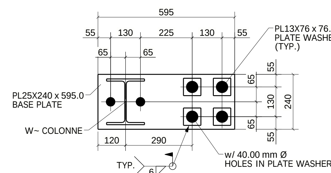
TYPE-10 (04-LOCATION) (REF : PB-1-B-4/S-170)
