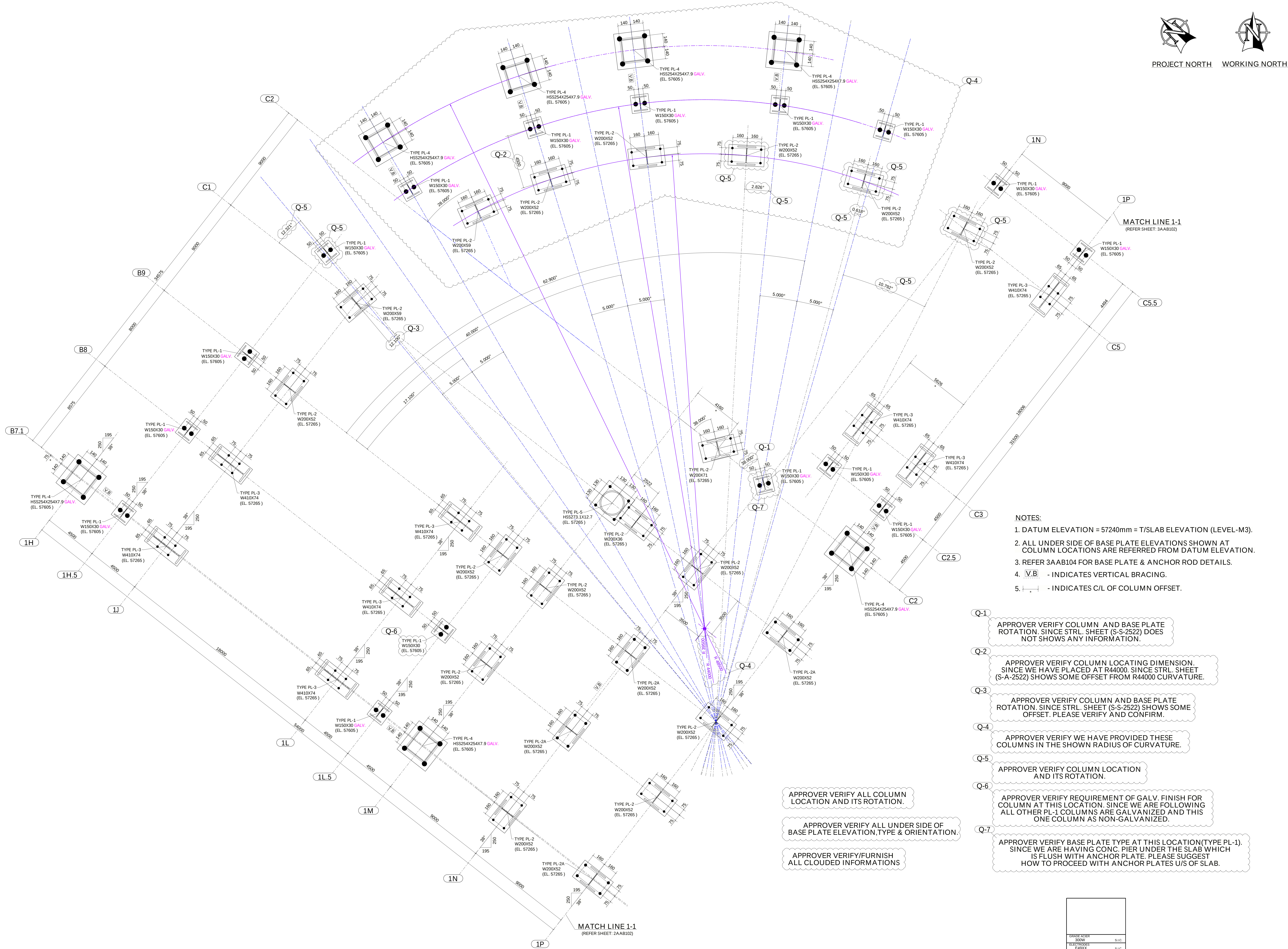
PARTIAL ANCHOR BOLT SETTING PLAN (LEVEL-M3) (SECTOR-A) (REFER SHEET: S-A-2522)
