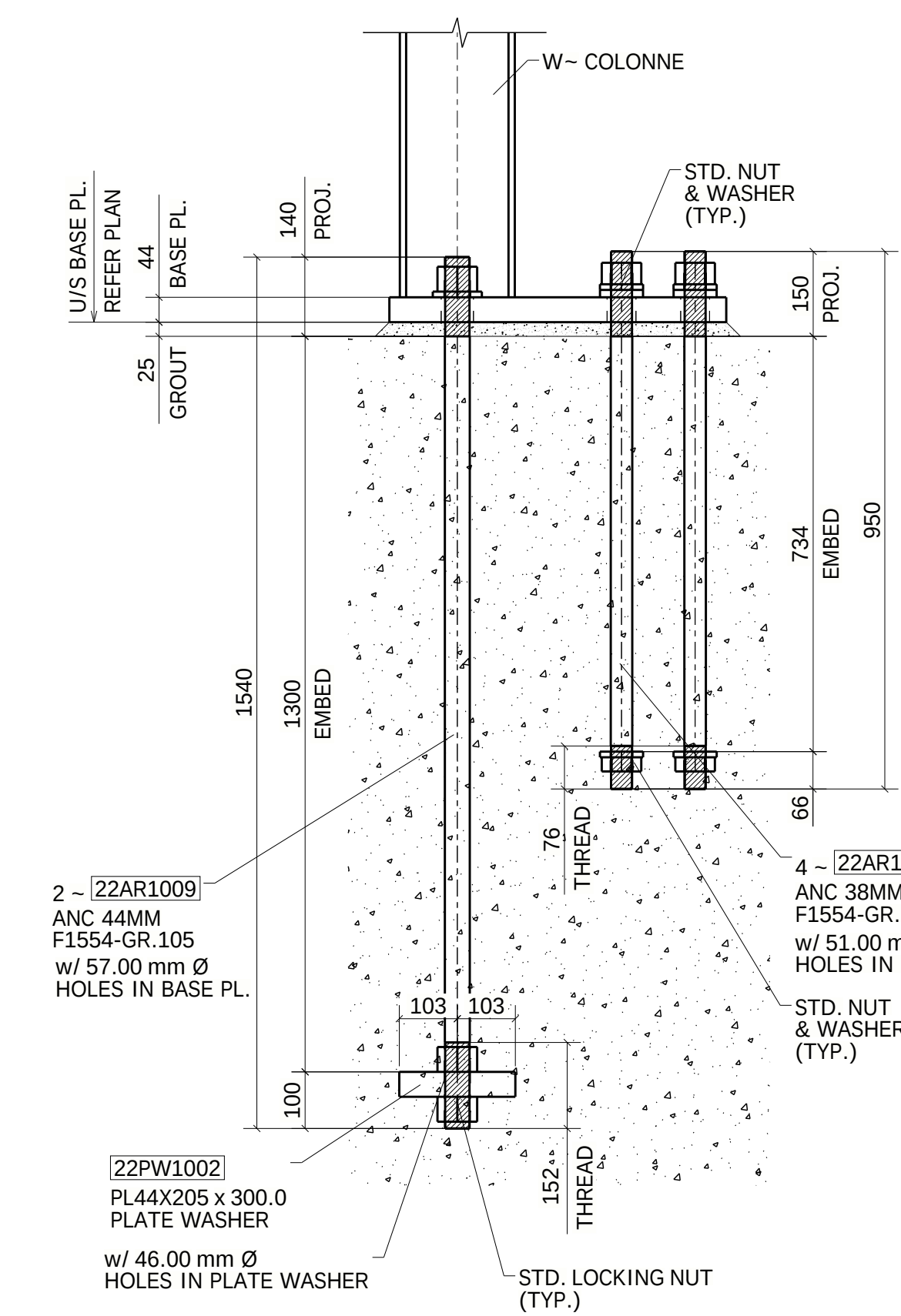
TYPE-11 (03-LOCATIONS) (REF : PB-1-B-6/S-170)
