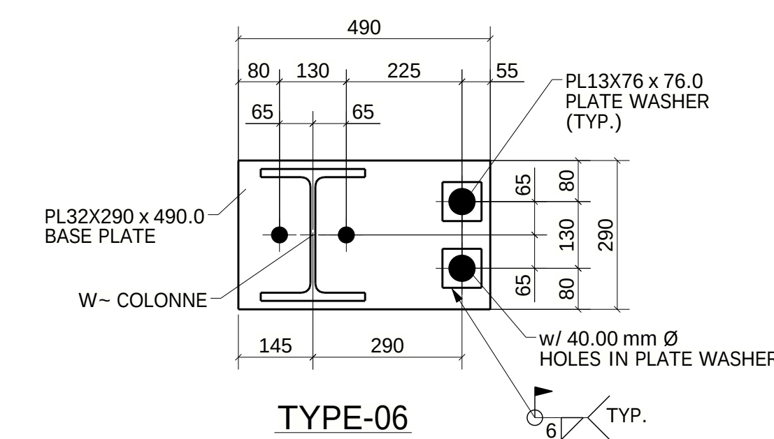
TYPE-06 (01-LOCATION) (REF : PB-2-A-2/S-170)
