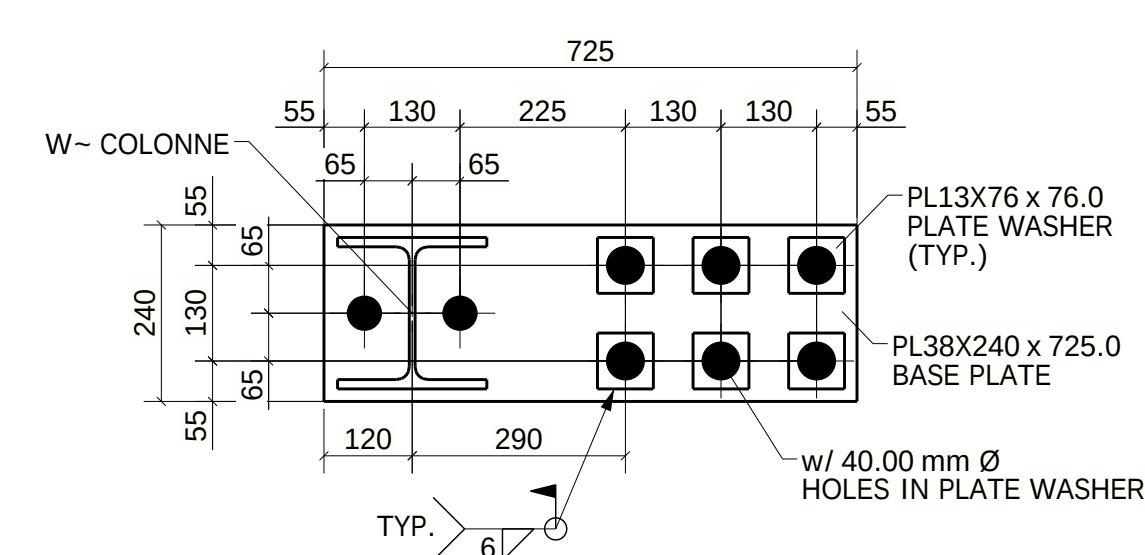
TYPE-12 (02-LOCATIONS) (REF : PB-1-C-6/S-170)
