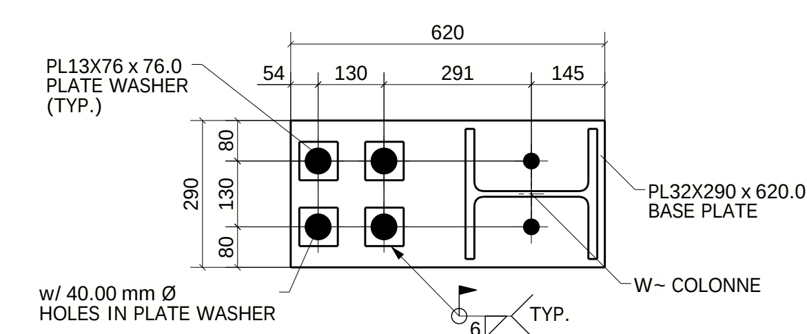
TYPE-05 (03-LOCATION) (REF : PB-2-A-4/S-170)
