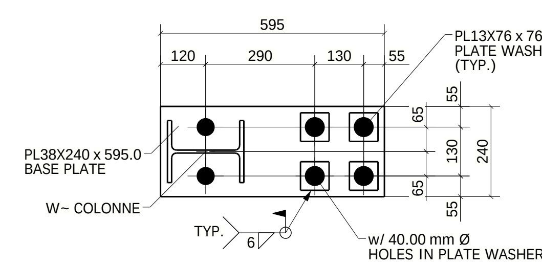
TYPE-18A (01-LOCATION) (REF : PB-1-C-4/S-170)
