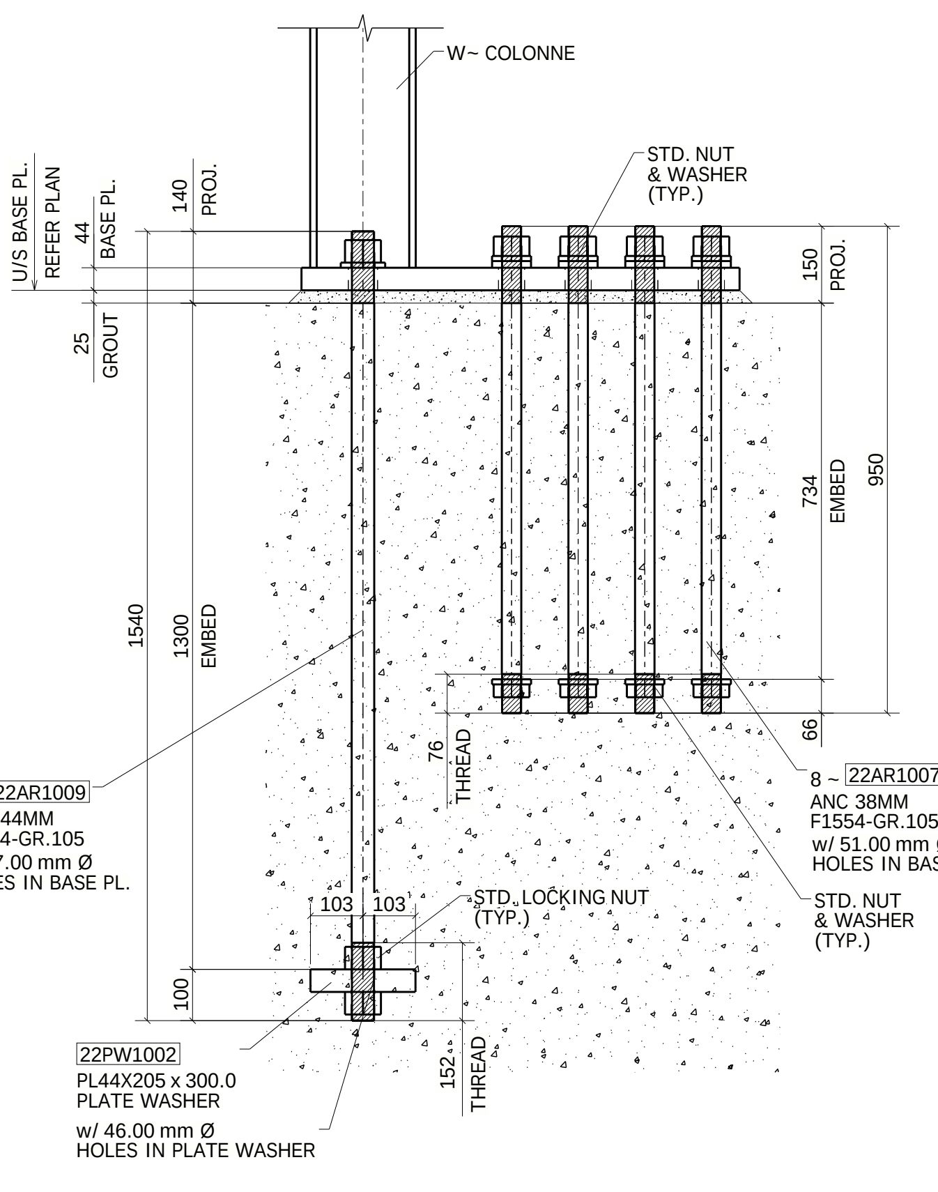
TYPE-12 (02-LOCATIONS) (REF : PB-1-C-6/S-170)
