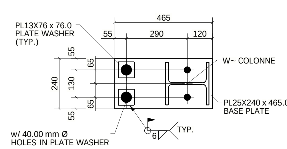
TYPE-07A (03-LOCATION) (REF : PB-1-A-2/S-170)
