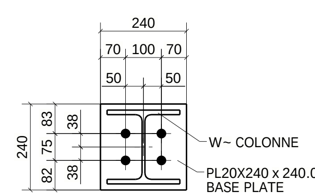
TYPE-01 (123-LOCATION) 119-LOCATION-NO PAINT (476 ANCHORS) 4-LOCATION- GALVANIZED (16 ANCHORS) (REF : PB-3/S-170)
