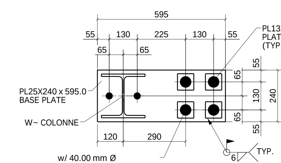
TYPE-08 (06-LOCATION) (REF : PB-1-A-4/S-170)
