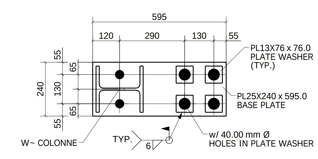
TYPE-10A (02-LOCATION) (REF : PB-1-B-4/S-170)
