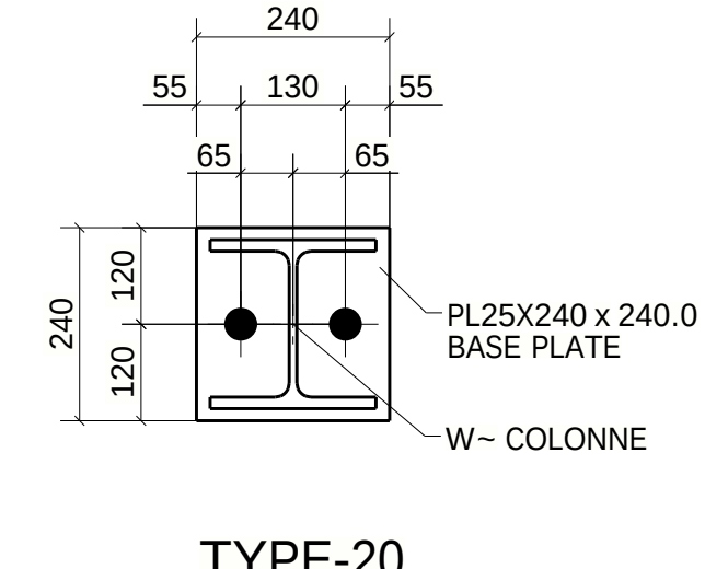
TYPE-20 (01-LOCATION) (REF : PB-1-B-0/S-170)
