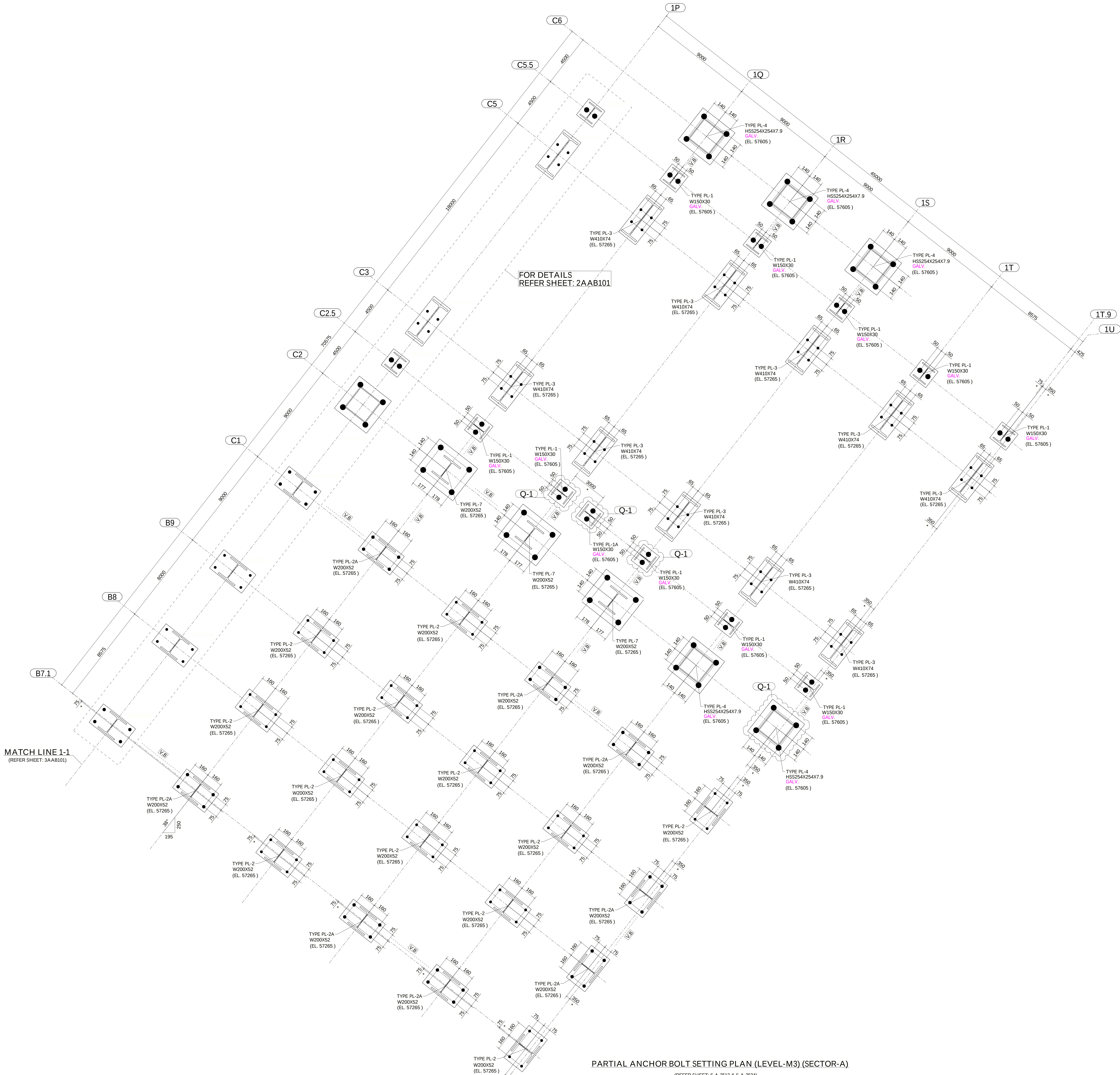
PARTIAL ANCHOR BOLT SETTING PLAN (LEVEL-M3) (SECTOR-A) (REFER SHEET: S-A-2512 & S-A-2534)
