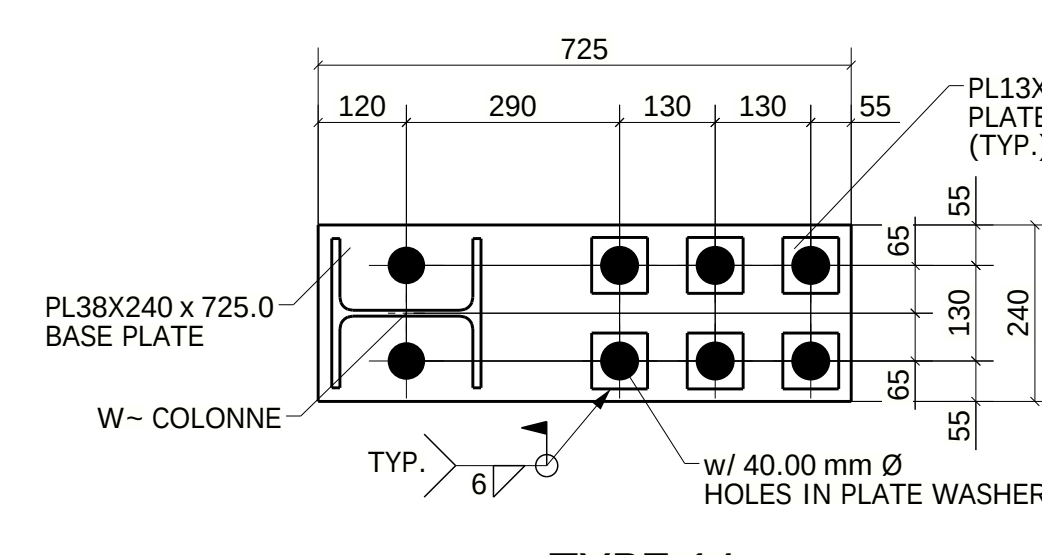
TYPE-14 (06-LOCATIONS) (REF : PB-1-D-6/S-170)
