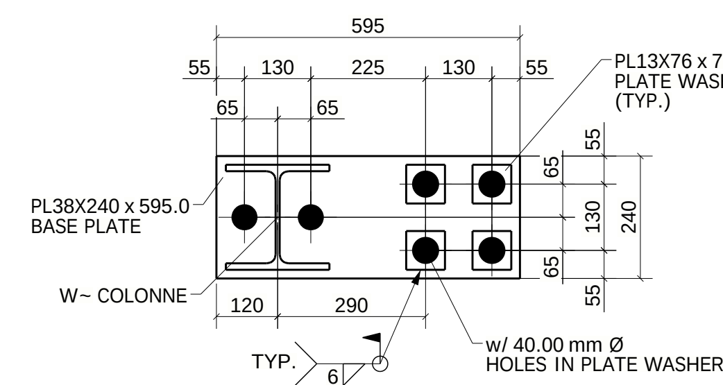
TYPE-13 (01-LOCATION) (REF : PB-1-D-4/S-170)
