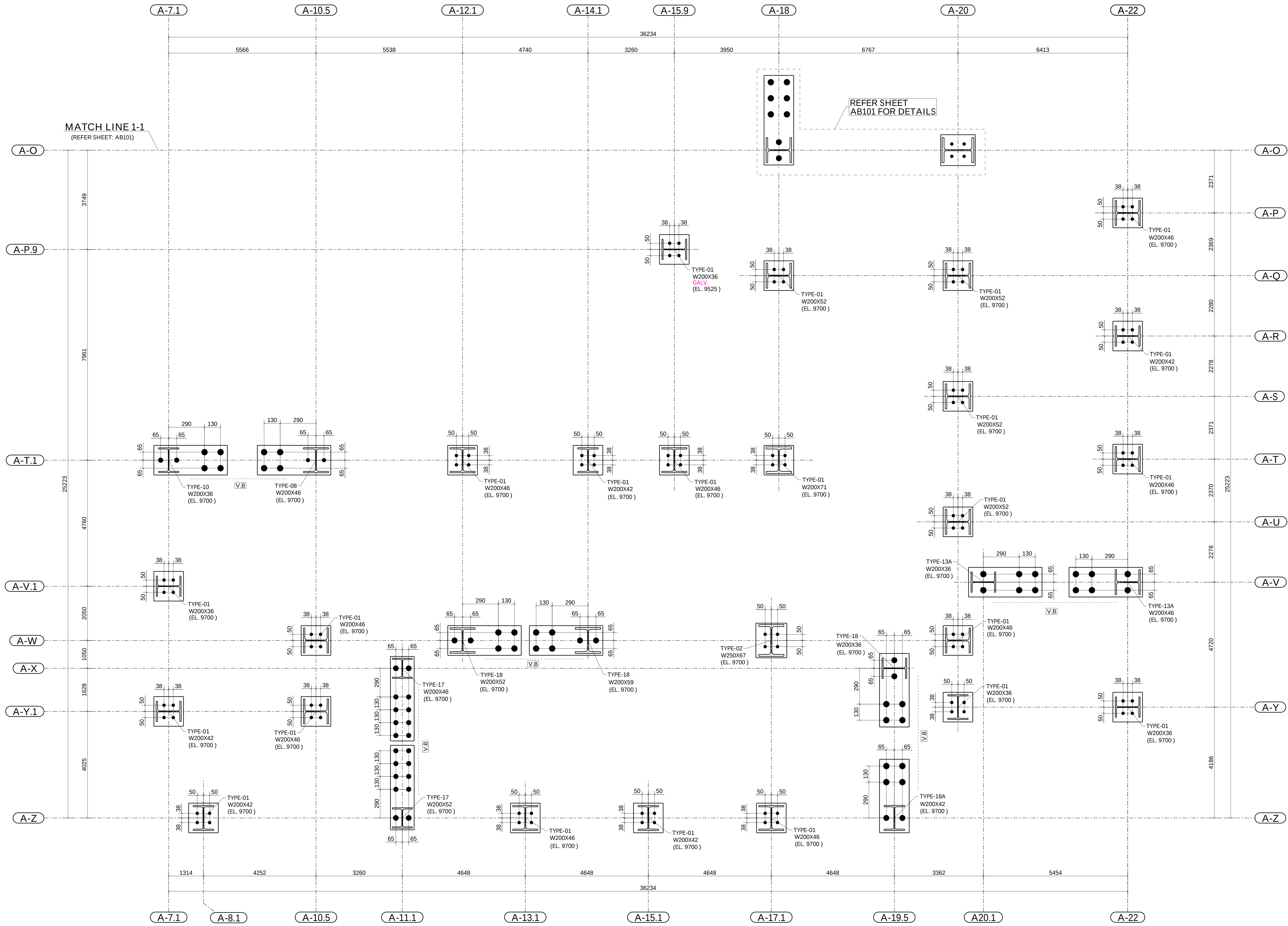
DETAIL-B AB-100 PARTIAL ANCHOR BOLT SETTING PLAN (SECTOR-A) (REFER SHEET S-152A)
