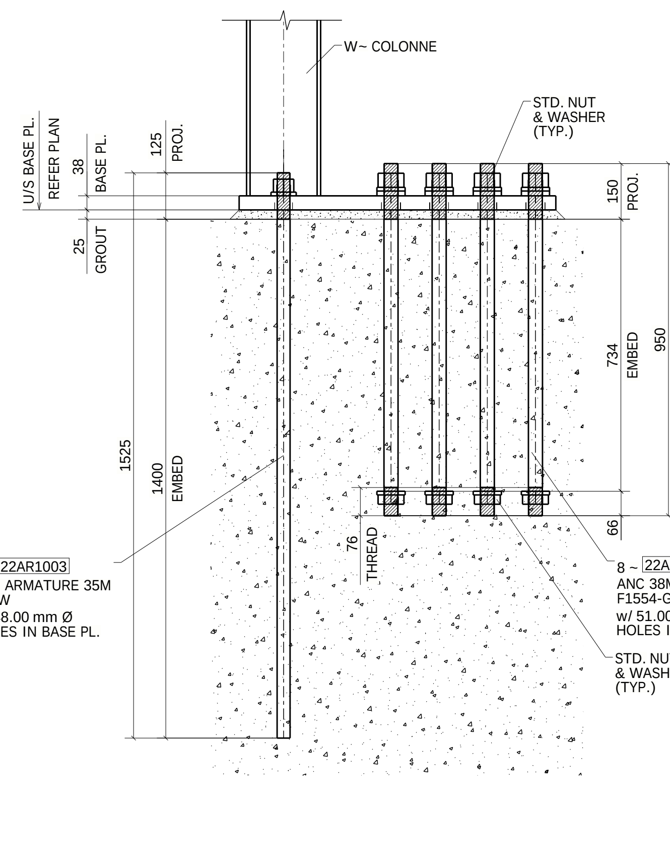
TYPE-14 (06-LOCATIONS) (REF : PB-1-D-6/S-170)
